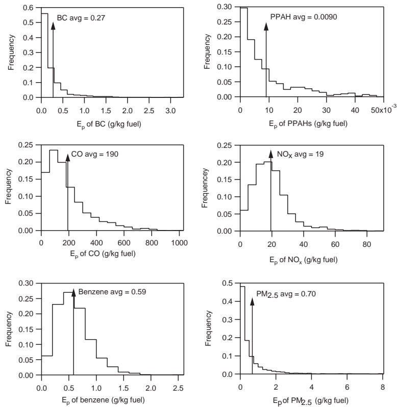
Fig. 3. Normalized distributions and averages of emission factors of BC, PPAH, CO, NO x , benzene, and PM 2.5 . Note that the range of the y-axis varies.
