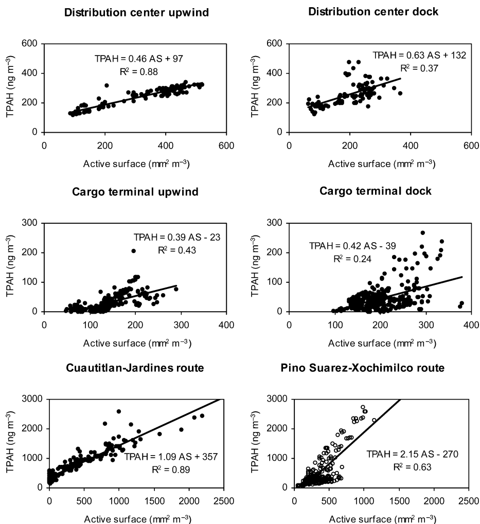
FIGURE 5. TPAH vs active surface (AS) area concentrations upwind and in the loading dock area of two diesel truck terminals and along two roadway routes. Solid and open circles represent data collected in October and June 2002, respectively. The Cuautitlan Izcalli-Jardines route was monitored on October 22, 2002, from inside a diesel truck cab, and the Pino Suarez-Xochimilco route was monitored during the morning commute on June 20 and 21, 2002, from inside an automobile.
